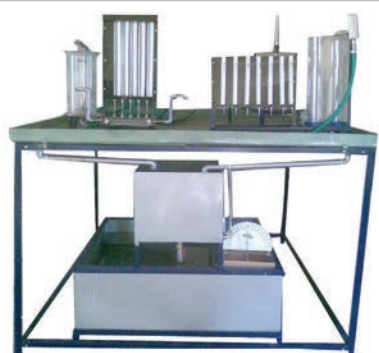
Hydraulic Bench
