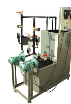
Series & Parallel Centrifugal Pump Test Rig
